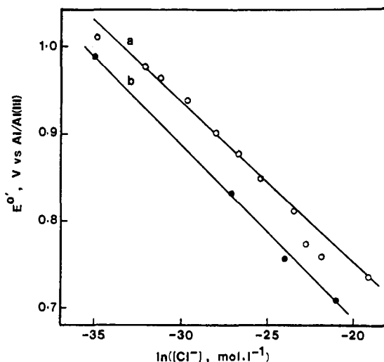
Figure 5. Plots of E^{\circ'} vs. \ln [Cl^-] for the Sb(III)/Sb couple in acidic melts: a, from potentiometry; b, from voltammograms of Sb(III) solutions on RGCDE obtained from a reverse scan (see text).
